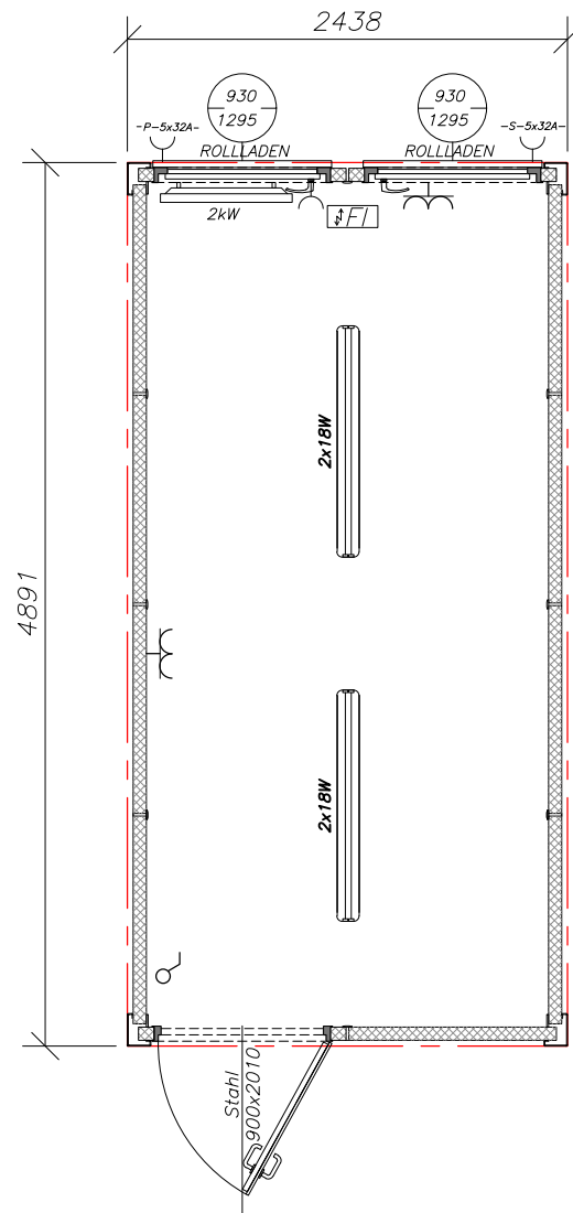
Containerplan MB16
