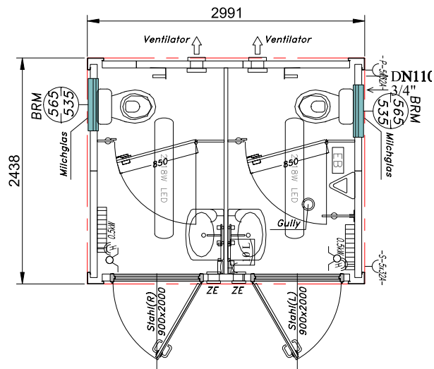
Containerplan MW 10
